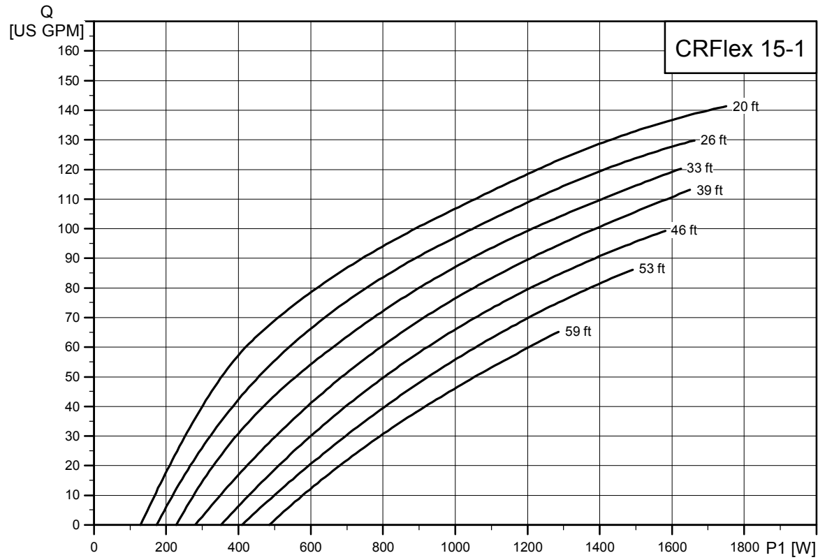
Fig. 32 Performance curves, CRFlex 15-1
