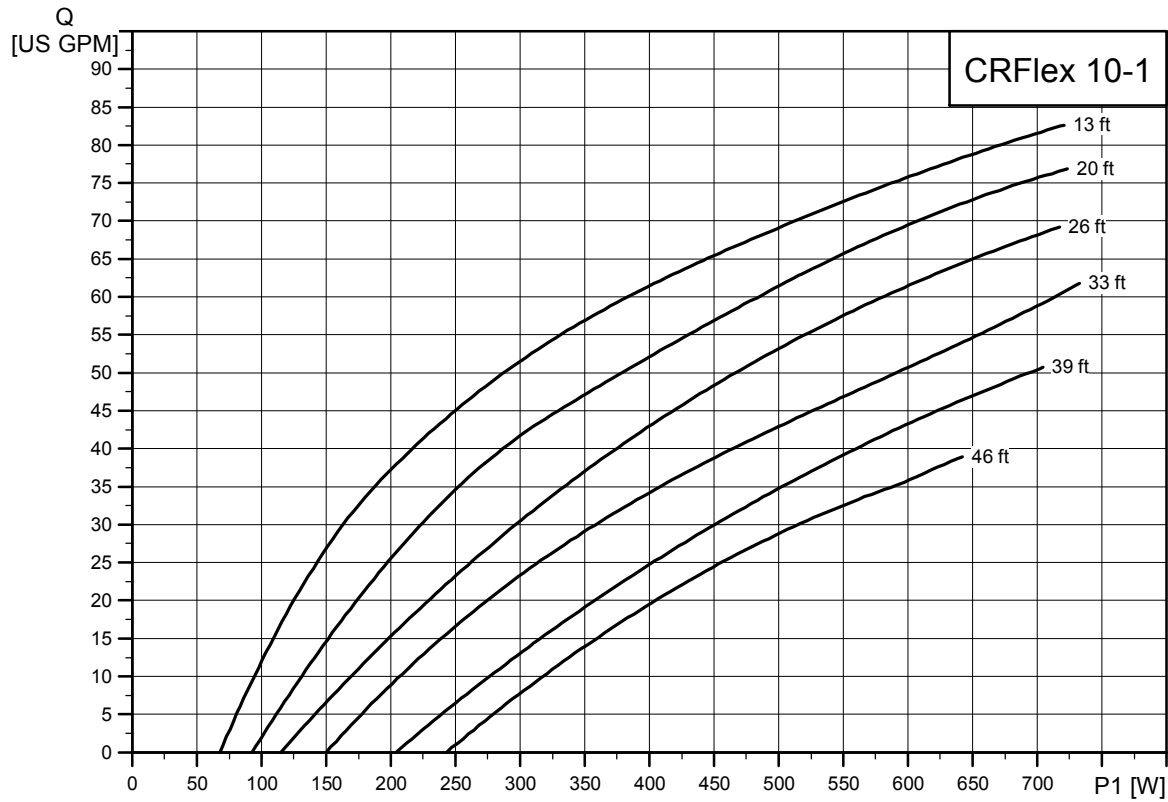
Fig. 30 Performance curves, CRFlex 10-1
